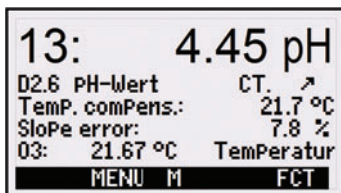
pH-Display, measured value with automatic temperature compensation
